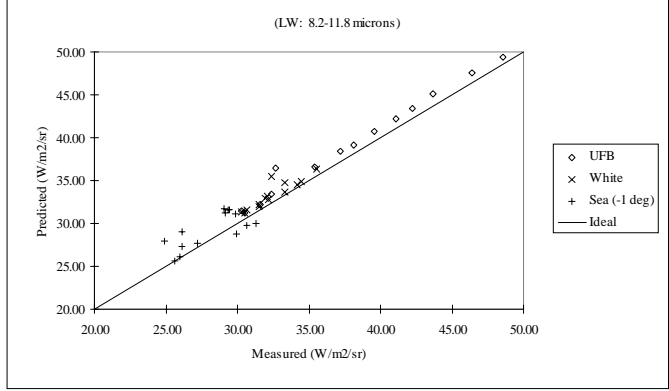
Figure 9: Predicted in-band radiance.
