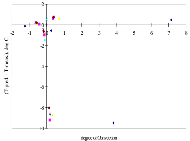
Figure 8: Sensitivity of panel temperature (no-sun) to convection.
