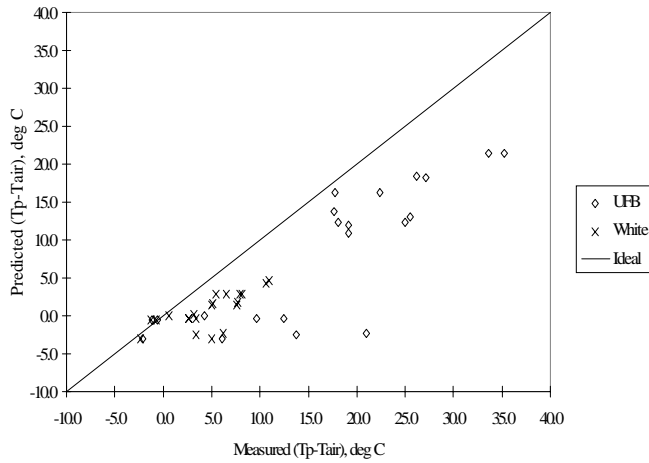
Figure 5: Predicted panel contrast temperatures.
