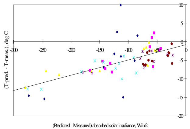
Figure 7: Effect of solar irradiance prediction error.
