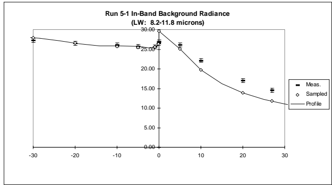
Figure 11: Background radiance profiles about the horizon on 15 May, 10:20 AM.
