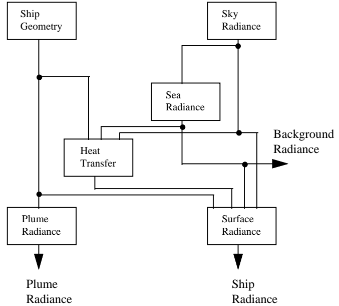
Figure 3: Block diagram illustrating sub-models of SHIPIR.
