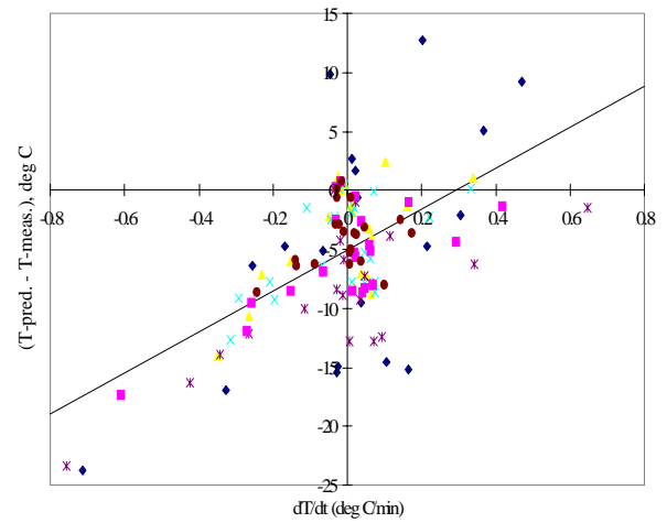
Figure 6: Effect of non-thermal equilibrium on temperature prediction.
