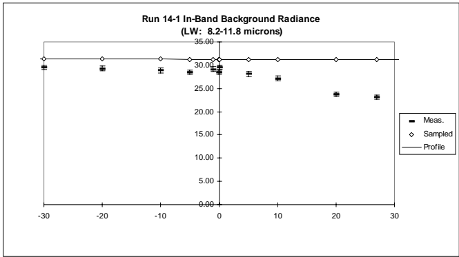
Figure 12: Background radiance profiles about the horizon on 27 May, 10:20 AM.
