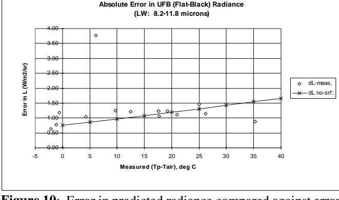
Figure 10: Error in predicted radiance compared against error in the approximation of spectral response.
